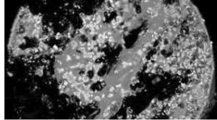
Back-scattered electron image of the spheroidal hiroshimaites sample in which the alloy was found. BINDI ET AL., SCI. ADV. 12, EAE8299 (2026)
